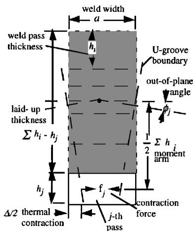
Fig. 2 Peaking from j th filler pass.
