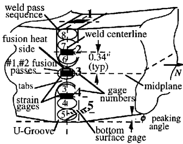
Fig. 3 Strain instrumentation.
